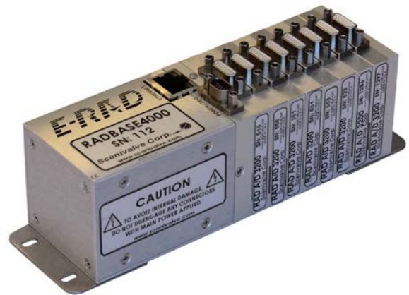
RADBASE4000 with 8 RAD A/D3200s
