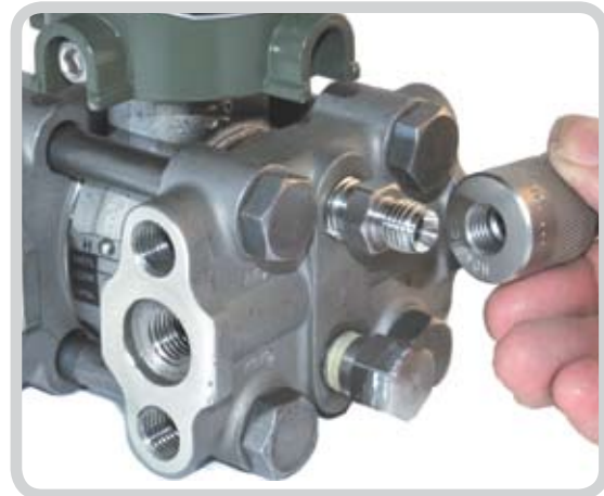
MET Style for External Threads
